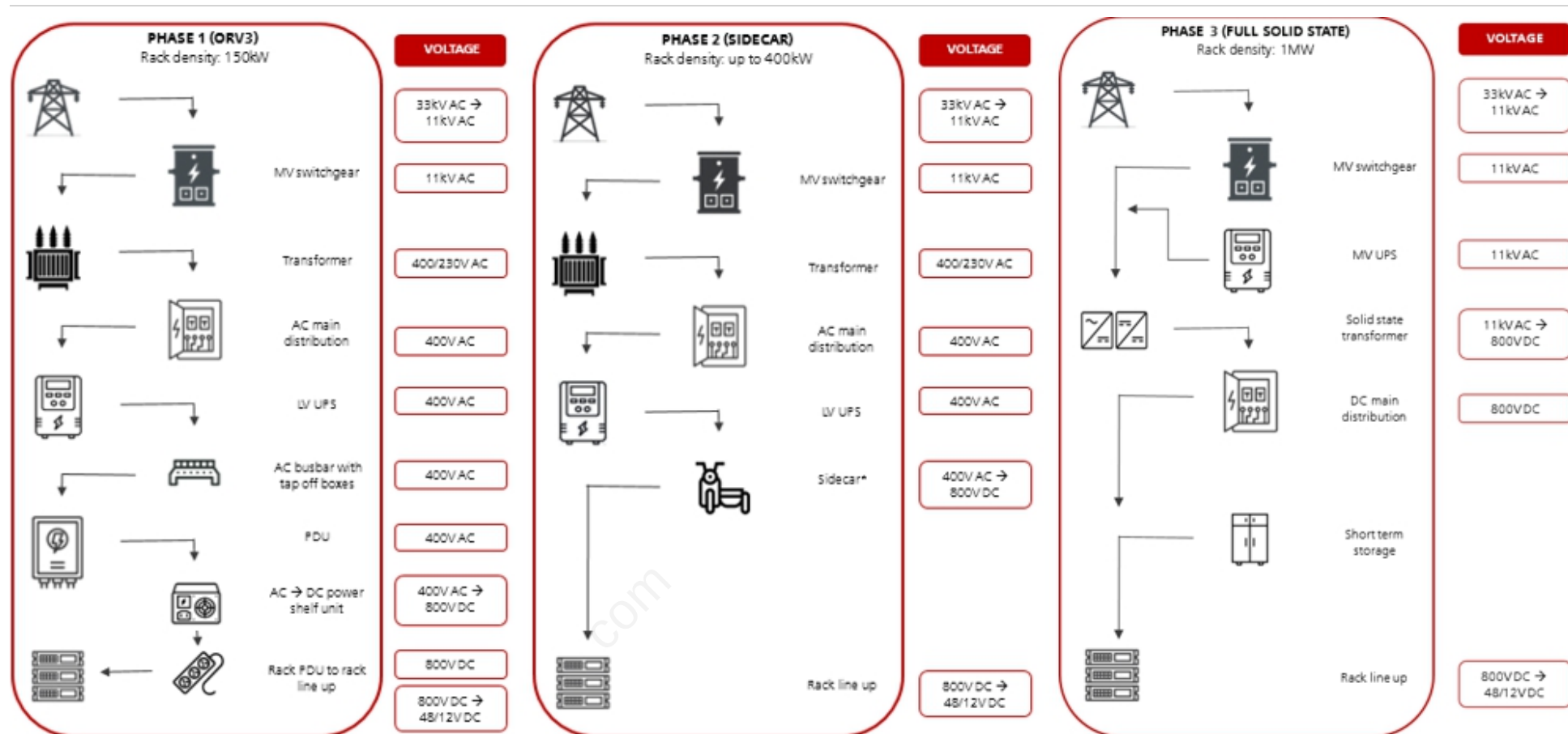
Figure 2: Three phases of 800V DC architecture
