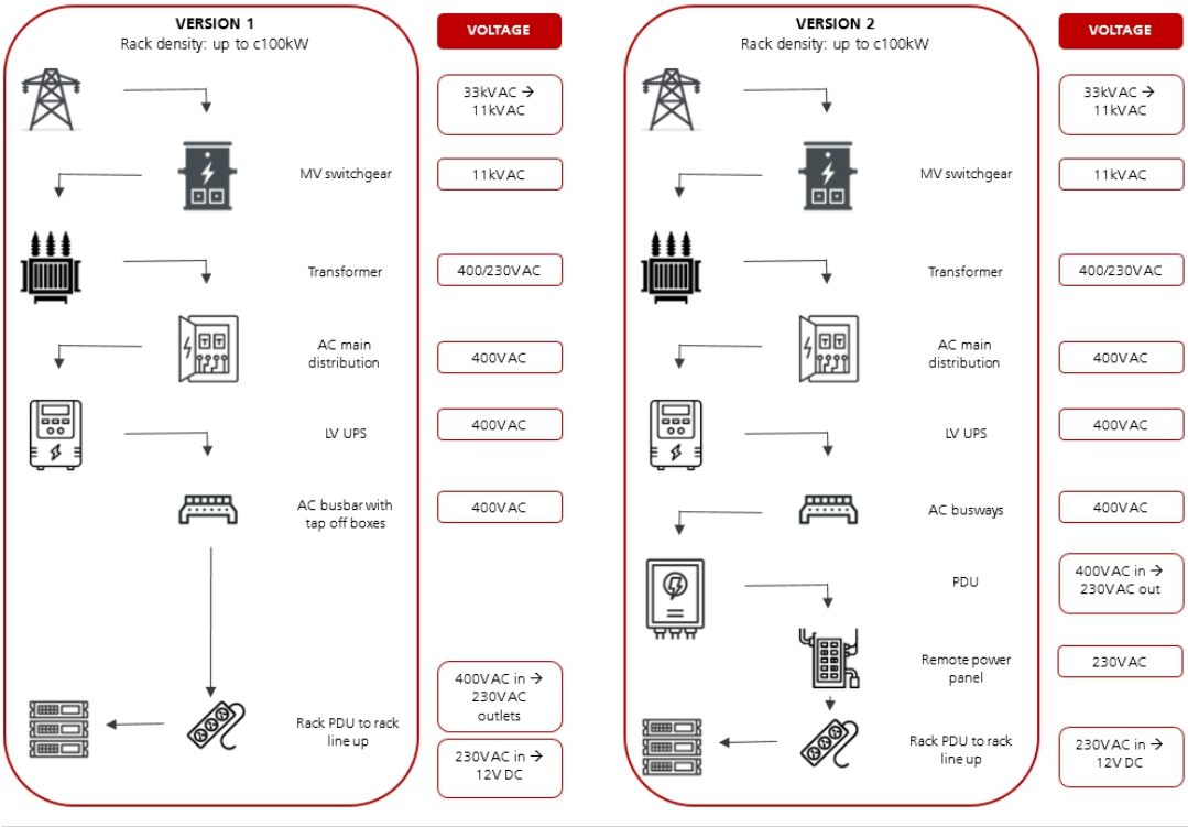
Figure 1: Data Centre architecture available today
